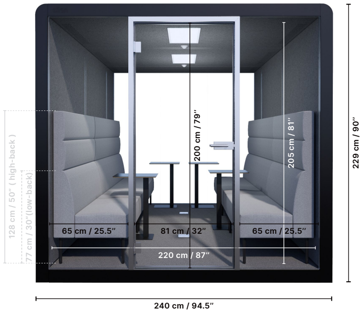
Space 4.5 ▲ front view
