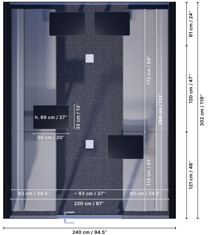
Space 4.5 ▲ top view
