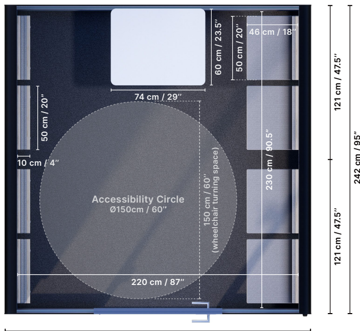
Space 4 Hybrid ▲ top view
