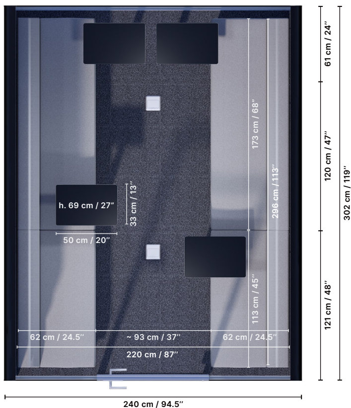
Space 4.5 ▲ top view
