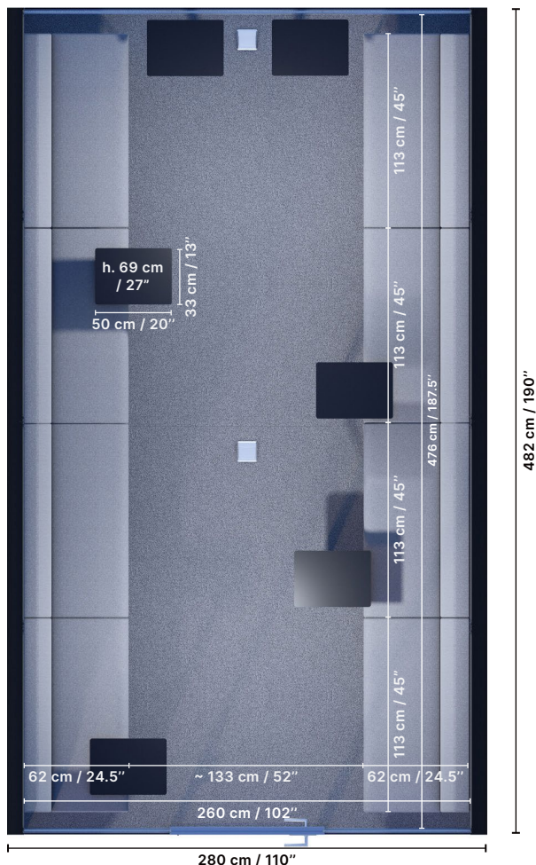
Space Max 2X ▶ top view
